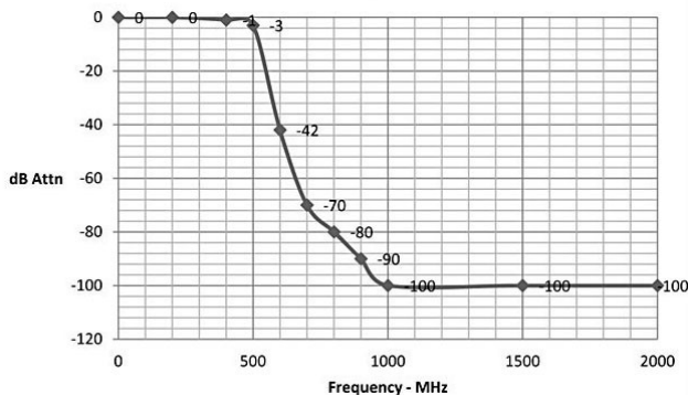
JRE LAN-2 RJ-45 Ethernet Filtered Interface Adapter
