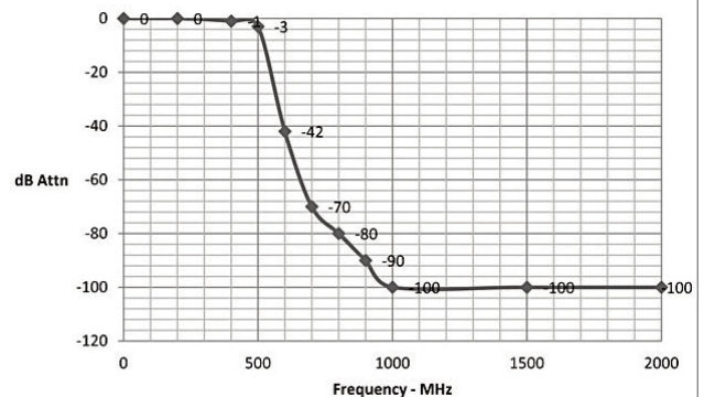
JRE LAN-2 RJ-45 Ethernet Filtered Interface Adapter
